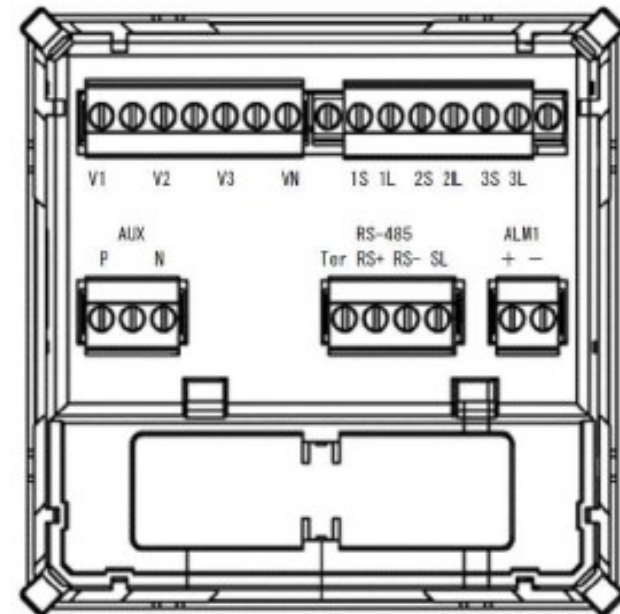
Connector Pinouts
