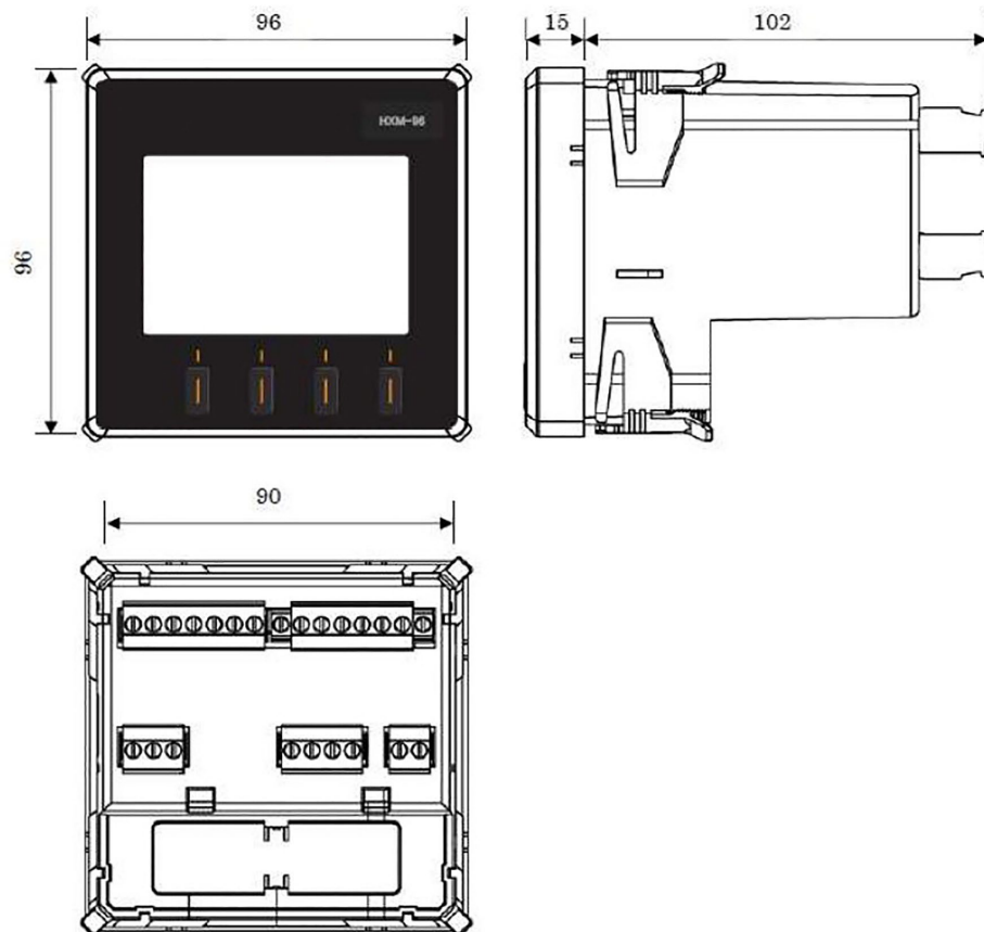
Outline Dimensional Drawing
